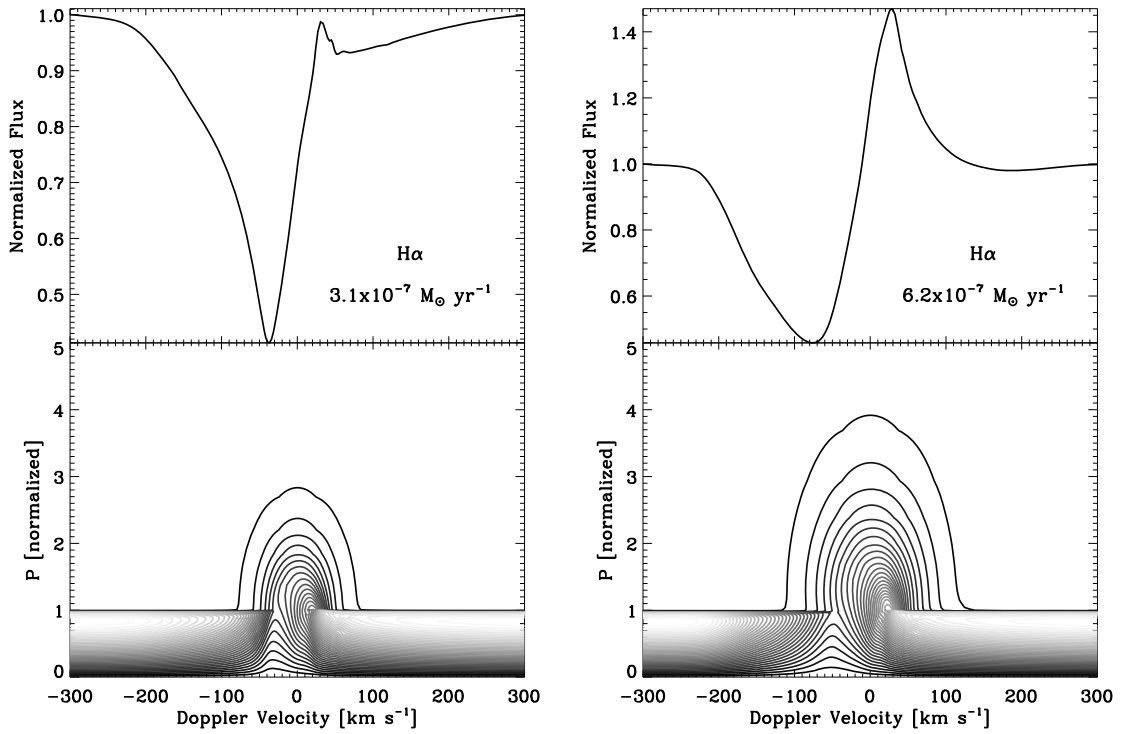
Fig. 6. Left: In the bottom panel, we show a contour plot of the quantity P \times I(P) as a function of Doppler velocity and impact parameter P for H\alpha , computed with CMFGEN using the stellar parameters of Deneb and a mass-loss rate value of 3.1 \times 10^{-7} M_{\odot} \text{ yr}^{-1} , corresponding to the best-fit model. This figure illustrates the distribution of intensity with impact parameter, and in particular serves to infer the regions that contribute significant flux to the line, and hence the spatial extent of the H\alpha line-formation region. In the top panel, we show the corresponding normalized synthetic flux in H\alpha . Right: same as left, but now for a mass-loss rate value of 6.2 \times 10^{-7} M_{\odot} \text{ yr}^{-1} . Notice the sizable change in profile morphology, echoing the change in the extent of the line-formation region.
