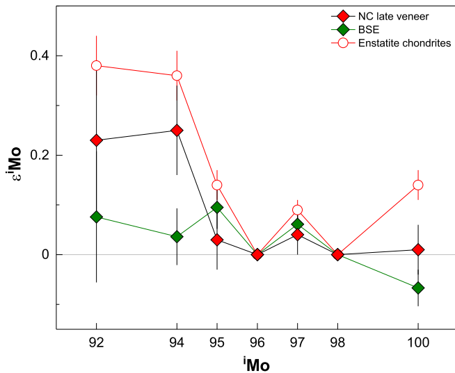
Fig. 6. \epsilon^1\text{Mo} values of a hypothetical NC late veneer defined by the x -axis intercepts of the Mo-Ru correlation (Table S3). Results of the regressions using all NC meteorites (except brachinites) and the OC L2 leachate are shown for comparison (Render et al., 2017; Budde et al., 2019). For s - and r -process nuclides ( ^{95}\text{Mo} , ^{97}\text{Mo} , and ^{100}\text{Mo} ) the BSE and the hypothetical NC late veneer have indistinguishable Mo isotopic compositions. However, for the two p -process nuclides ( ^{92}\text{Mo} and ^{94}\text{Mo} ) the inferred composition of the hypothetical NC late veneer is significantly different from BSE. Uncertainties on the NC late veneer values are 95% c.i., as calculated by the linear regression (Table S3).
