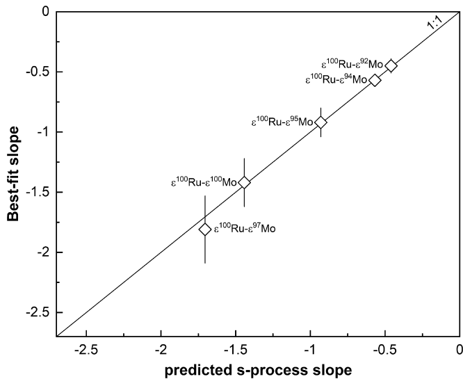
Fig. 5. Plot of the best-fit \epsilon^{100}\text{Ru} vs. \epsilon^i\text{Mo} slopes defined by the linear regressions of all NC meteorites (except brachinites) and the OC L2 leachate versus the predicted slopes of s -process mixing lines (Table S3). Predicted s -process slopes are based on data for presolar SiC grains (Arlandini et al., 1999; Savina et al., 2004; Stephan et al., 2019) and were calculated using equations described in Dauphas et al. (2004). Best-fits were calculated using the York method and the software suite OriginPro (OriginLab, Northampton, MA). Uncertainties are 95% c.i. as calculated by the linear regression (Table S3).
