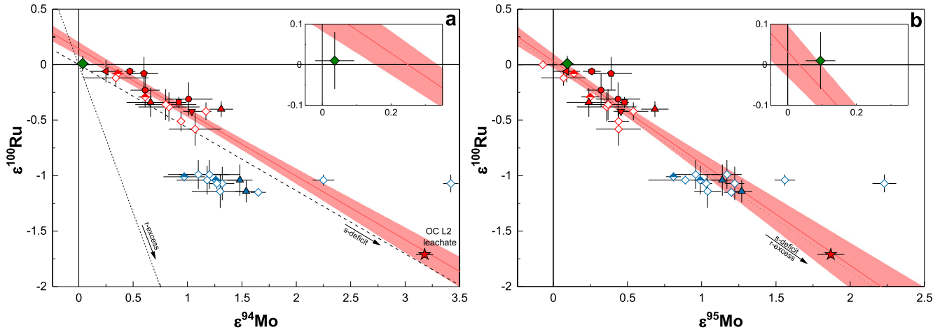
Fig. 4. Best-fits of the Mo-Ru isotope correlation for NC meteorites in (a) \epsilon^{100}\text{Ru} vs. \epsilon^{94}\text{Mo} (b) \epsilon^{100}\text{Ru} vs. \epsilon^{95}\text{Mo} space. The L2 acid leachate of the ordinary chondrite NWA 2458 (red star ‘OC L2 leachate’) falls exactly on the Mo-Ru correlation line defined by the NC meteorites. Red solid lines are linear regressions of the NC data for \epsilon^{100}\text{Ru} vs. \epsilon^{94,95}\text{Mo} including all NC meteorites (except brachinites) and the OC L2 leachate (shaded red area is 95% c.i. of best-fit). (a) In the \epsilon^{100}\text{Ru} vs. \epsilon^{94}\text{Mo} plot, the Mo-Ru correlation defines x -axis intercepts that are resolved from zero (Table S3) and CC meteorites do not plot on the correlation defined by NC meteorites. (b) In the \epsilon^{100}\text{Ru} vs. \epsilon^{95}\text{Mo} plot, the x -axis intercepts are not resolved from zero (Table S3) and the CC cluster falls on the correlation line defined by NC meteorites. Symbols and data of bulk meteorites as in Fig. 3 (and Table S2, S4). Data for BSE from Bermingham and Walker (2017) and Budde et al. (2019). Best-fits were calculated using the York method and the software suite OriginPro (OriginLab, Northampton, MA).
