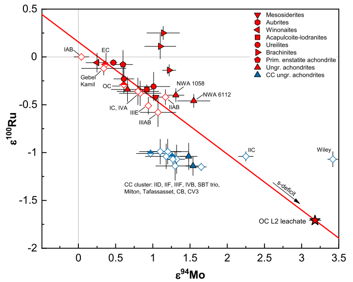
Fig. 3. Diagram of \epsilon^{100}\text{Ru} vs. \epsilon^{94}\text{Mo} for samples of this study together with literature data for chondrites (half-open diamonds) and iron meteorites (open diamonds). Except for brachinites, NC meteorites (red symbols) show a broad correlation between \epsilon^{94}\text{Mo} and \epsilon^{100}\text{Ru} , whereas CC meteorites (blue symbols) have indistinguishable \epsilon^{100}\text{Ru} of \sim -1 , with most plotting in a cluster at \epsilon^{94}\text{Mo} \approx 1.3 . The red solid line is the s -process mixing line defined by NC meteorites as described in sect. 4.2 and Fig. 4. Literature data from Fischer-Gödde et al. (2015), Render et al. (2017), Fischer-Gödde and Kleine (2017), Burkhardt et al. (2017), Poole et al. (2017), Birmingham et al. (2018), Budde et al. (2019), Worsham et al. (2019), and Hilton et al. (2019).
