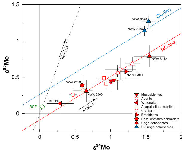
Fig. 1. Diagram of \epsilon^{95}\text{Mo} vs. \epsilon^{94}\text{Mo} for samples of this study. In this plot, the Mo isotope dichotomy between carbonaceous (CC, blue) and non-carbonaceous (NC, red) materials is defined by two parallel lines with identical slopes (Budde et al., 2019). Samples from both groups have variable s -process deficits relative to the bulk silicate Earth (BSE) and plot along each line. The offset between the lines reflects an approximately constant r -excess in the CC reservoir. Two of the ungrouped primitive achondrites (NWA 8548, NWA 6926) plot on to the CC-line, whereas all other samples of this study plot on the NC-line. Open symbols represent samples for which Mo isotopic data are reported in Budde et al. (2019), and which were investigated for Ru isotopes in this study. For samples shown with closed symbols, both Mo and Ru isotopic data were obtained in this study. Slopes of NC-, CC-, and r -process mixing lines as well as the composition of the BSE are from Budde et al. (2019). (For interpretation of the colors in the figure(s), the reader is referred to the web version of this article.)
