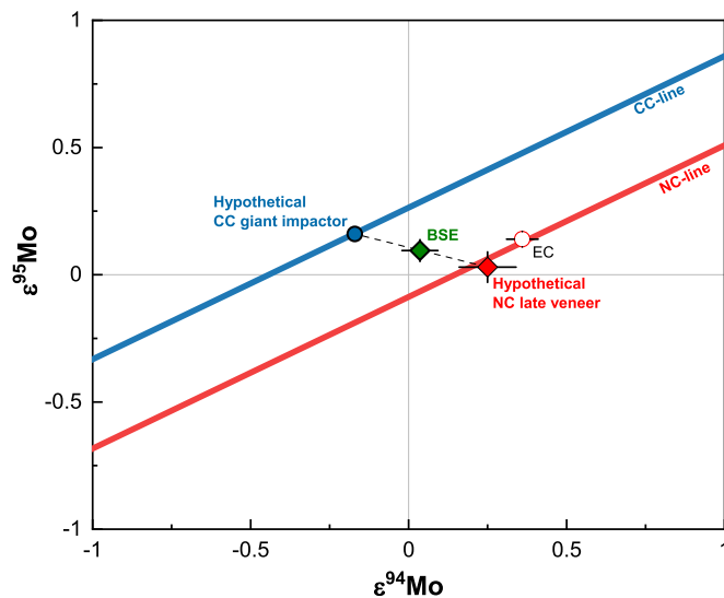
Fig. 7. Diagram of \epsilon^{95}\text{Mo} vs. \epsilon^{94}\text{Mo} illustrating the position of the BSE between the NC- and CC-lines (Budde et al., 2019). One possible endmember scenario for Earth's late-stage accretion involving a NC late veneer and a CC Moon-forming giant impactor is shown. The Mo isotopic composition of a hypothetical NC late veneer is given by the x -axis intercepts of the \epsilon^{100}\text{Ru} vs. \epsilon^1\text{Mo} correlations for NC meteorites (see Fig. 6) and falls exactly on the NC-line (red diamond). Based on this hypothetical late veneer composition and the BSE composition, the Moon-forming impactor was a CC body and had a small excess in s -process nuclides relative to the BSE (blue circle).
