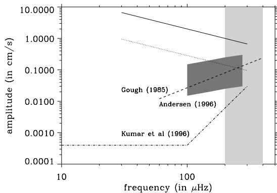
Figure 4. The black thin line is the limit for a singlet derived by Christensen-Dalsgaard (2002) from the upper limit given by Appourchaux et al. (2000) for a 2-year observing time. The dotted is the upper limit for a multiplet for a 10-year observing time scaled as in Eq. (1) assuming an improvement by a factor 3 with respect to a singlet. The thick black dotted-dashed and thick black dashed curves are the simplified version of the theoretical g-mode amplitude for l = 1 predicted by Gough (1985) and Kumar et al. (1996), respectively. The dark grey box shows the theoretical range of g-mode amplitude derived for l = 1 from calculation performed by Andersen (1996). The light grey box shows the location of the mixed modes.
