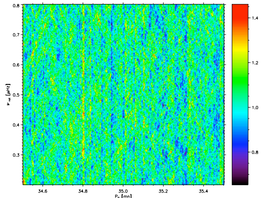
Figure 2. Total power in asymptotic g-mode frequencies as a function of the fundamental g-mode period P_0 and of rotational splitting for Blue SPM data. The total number of modes is about 100, the mean is 1 while the rms value is 0.1.
